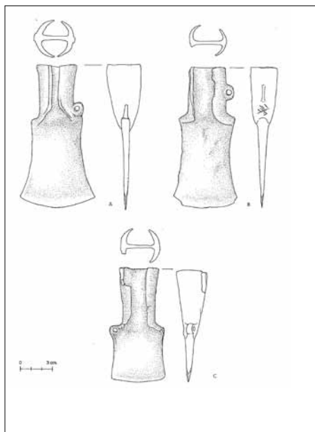
Fig. 18 a, b – Iron axes with eyelet from “Doss Castel” (Fai de la Paganella, Tn); c - iron axe from Borgo S. Pietro (Valsugana, Tn). (illustration from Marzatico F. 1997, p. 406)
